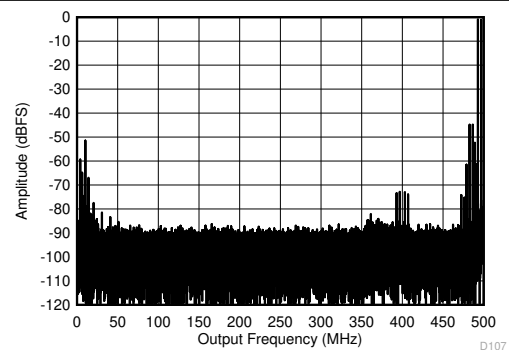
Figure 6-74. Two Tone FFT at 3498 MHz 10 MHz tone spacing, -7 dBFS per tone, Low power mode, 1000MSPS
