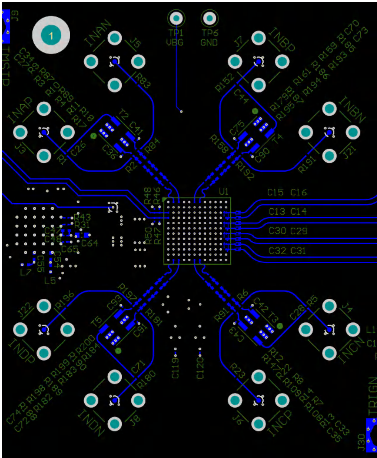
Figure 8-5. Top Layer Routing: Analog Inputs (INA±, INB±, INC±, IND±), TMSTP± and D[3:0]± Routing
