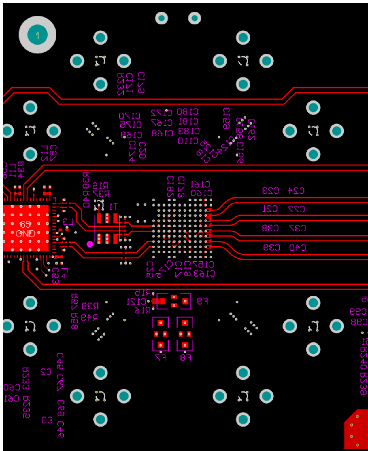
Figure 8-7. Bottom Layer Routing: CLK±, SYSREF and D[7:4]± Routing
