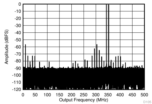
Figure 6-72. Two Tone FFT at 348 MHz 10 MHz tone spacing, -7 dBFS per tone, Low power mode, 1000MSPS
