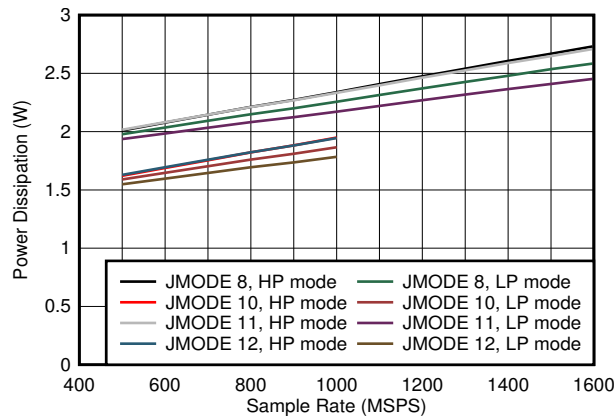
Low power background calibration mode Figure 6-81. Quad Channel, Power Dissipation vs F_S and JMODE 8 - 12
