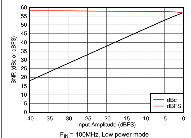
Figure 5-35. SNR vs A IN
