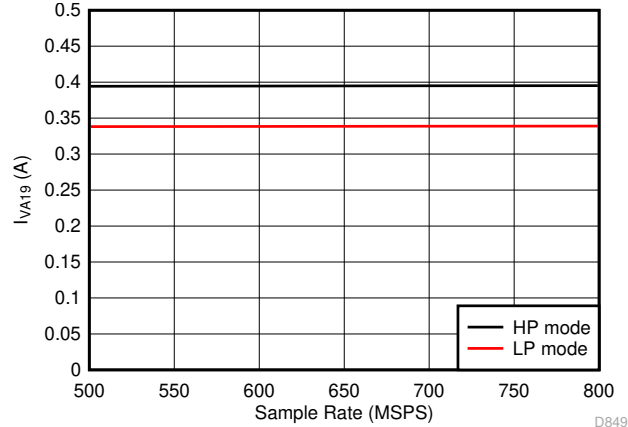
Figure 5-92. Dual Channel, I_{VA19} vs F_S
