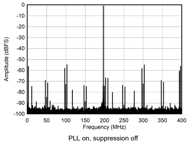
PLL on, suppression off Figure 5-16. Single Tone FFT at 997 MHz and -1dBFS
