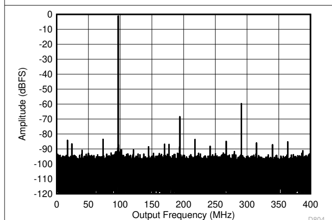
Figure 5-11. Single Tone FFT at 897 MHz and -1dBFS
