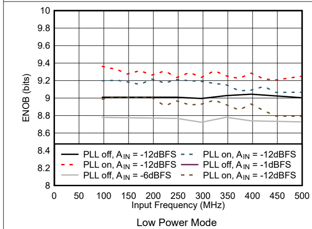
Figure 5-53. ENOB vs Input Frequency in Low Power Mode
