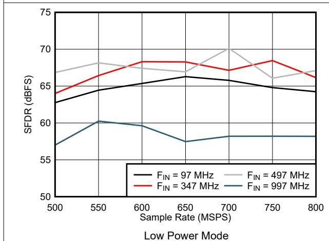
Figure 5-55. SFDR vs Sample Rate in Low Power Mode
