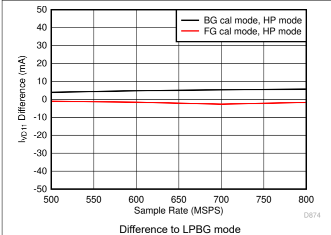
Figure 5-87. Quad Channel, I_{VD11} vs F_S over Modes
