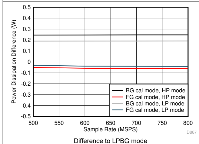
Figure 5-111. Single Channel, Power Dissipation vs F_S over Modes
