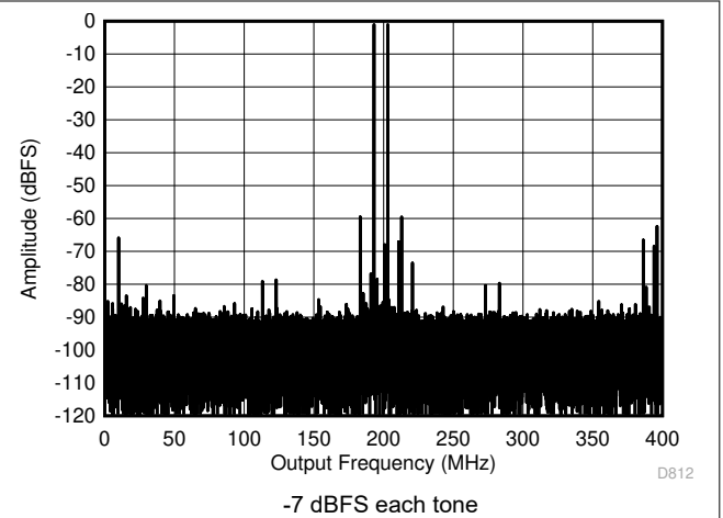
Figure 5-70. Two Tone FFT at 1798 MHz in Low Power Mode
