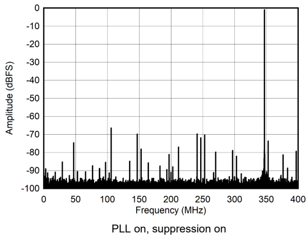
PLL on, suppression on Figure 5-15. Single Tone FFT at 347 MHz and -1dBFS
