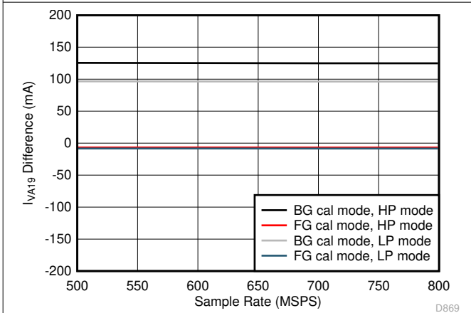
Figure 5-99. Dual Channel, I_{VA19} vs F_S over Modes
