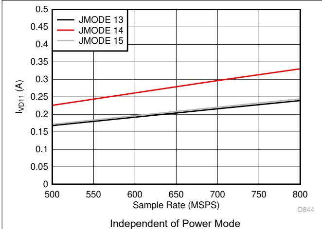
Figure 5-83. Quad Channel, I_{VD11} vs F_S for JMODES 13-15
