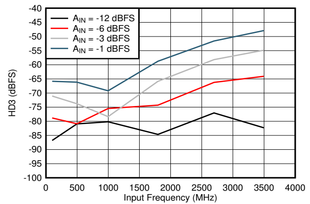
Figure 5-22. HD3 vs Input Frequency
