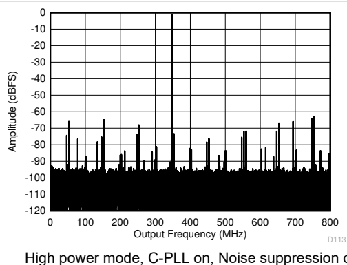
Figure 5-6. Single Tone FFT at 347MHz and -1dBFS
