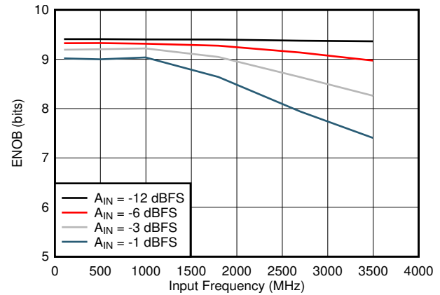
Figure 5-20. ENOB vs Input Frequency
