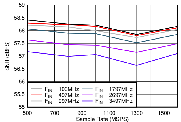
Figure 5-24. SNR vs Sample Rate
