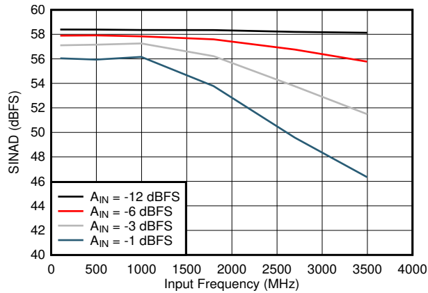
Figure 5-19. SINAD vs Input Frequency
