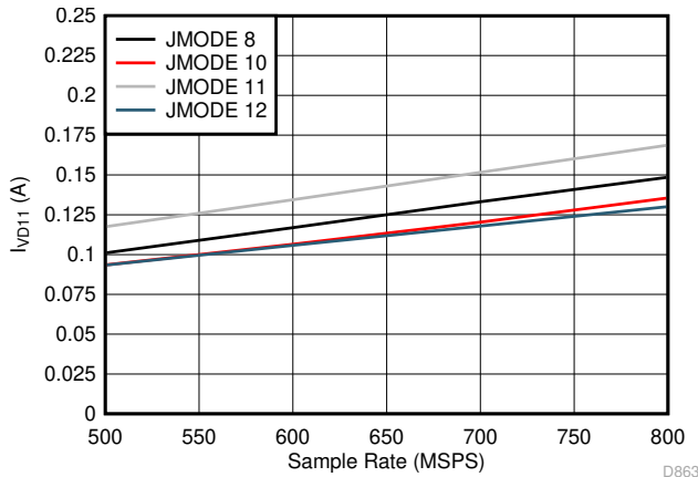
Figure 5-109. Single Channel, I_{VD11} vs F_S for JMODES 8 - 12
