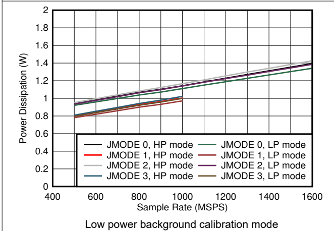
Figure 5-99. Single Channel, Power Dissipation vs F_S and JMODE 0 - 3
