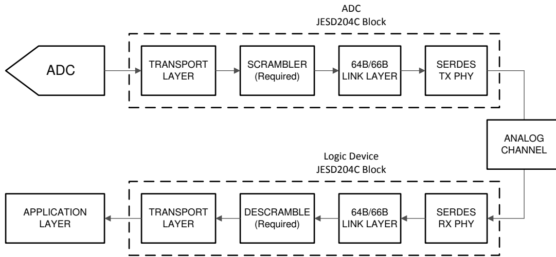
Figure 6-6. Simplified 64B/66B Encoded JESD204C Interface Diagram
