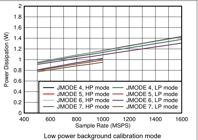
Figure 5-100. Single Channel, Power Dissipation vs F_S and JMODE 4 - 7
