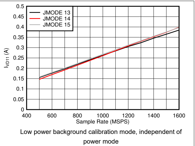
Figure 5-98. Dual Channel, Power Dissipation vs F_S and JMODE 13 - 15
