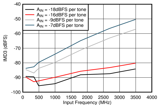
10MHz tone spacing, Low power mode, 1000MSPS
