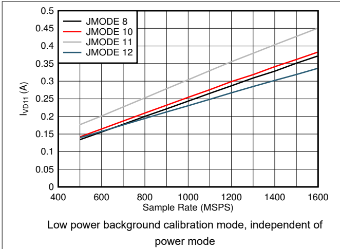
Figure 5-97. Dual Channel, Power Dissipation vs F_S and JMODE 8 - 12
