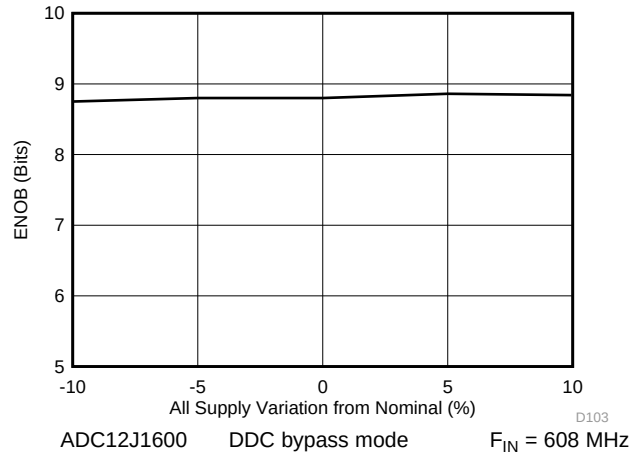
Figure 34. ENOB vs Supply Voltage
