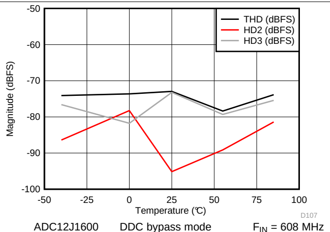
Figure 38. THD, H2, H3 vs Temperature
