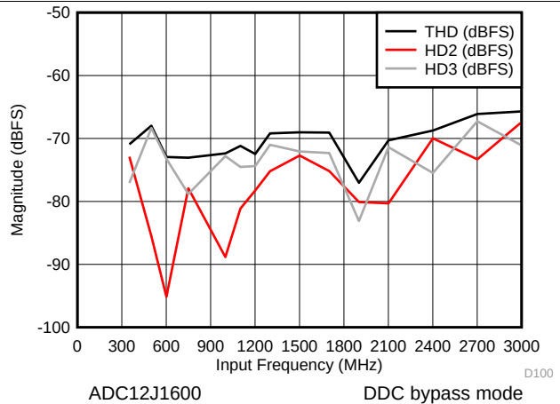
Figure 36. THD, H2, H3 vs Input Frequency
