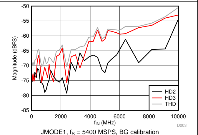
Figure 13. HD2, HD3, THD vs Input Frequency
