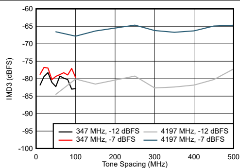
Figure 6-109. Dual Channel Mode: IMD3 vs Tone Spacing
