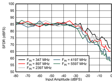
Figure 6-57. DES Mode: SFDR vs Input Amplitude and Frequency
