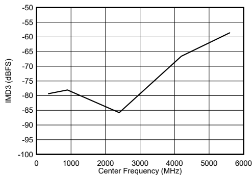
Figure 6-105. Dual Channel Mode: IMD3 vs Input Frequency
