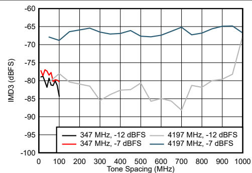
Figure 6-108. DES Mode: IMD3 vs Tone Spacing
