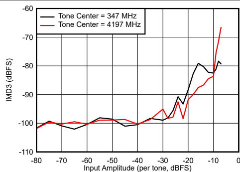
Figure 6-107. Dual Channel Mode: IMD3 vs Input Amplitude
