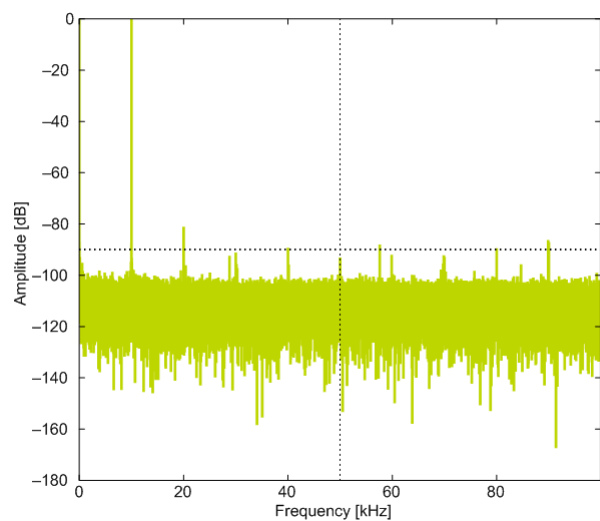
1.25 V Reference
