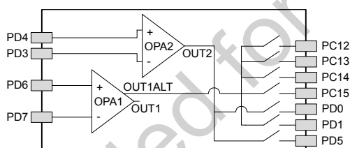
Figure 5.2. Opamp Pinout
