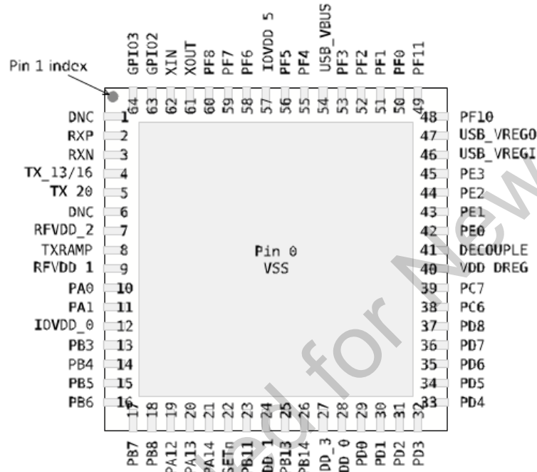
Figure 5.1. Pinout (top view, not to scale)
