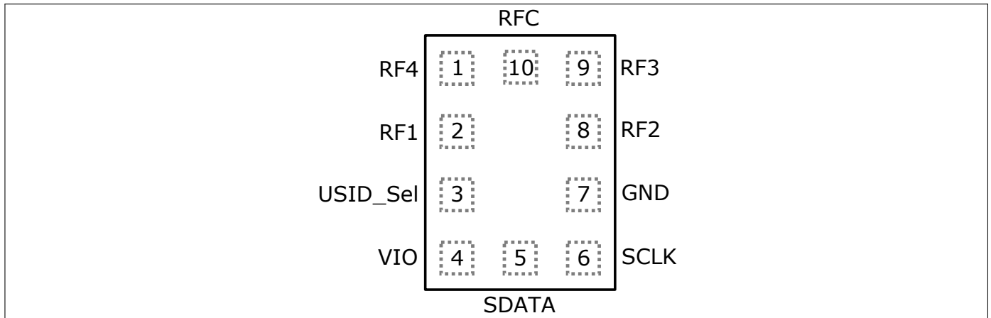
Figure 5: BGSA144ML10 Pin Configuration (top view)
