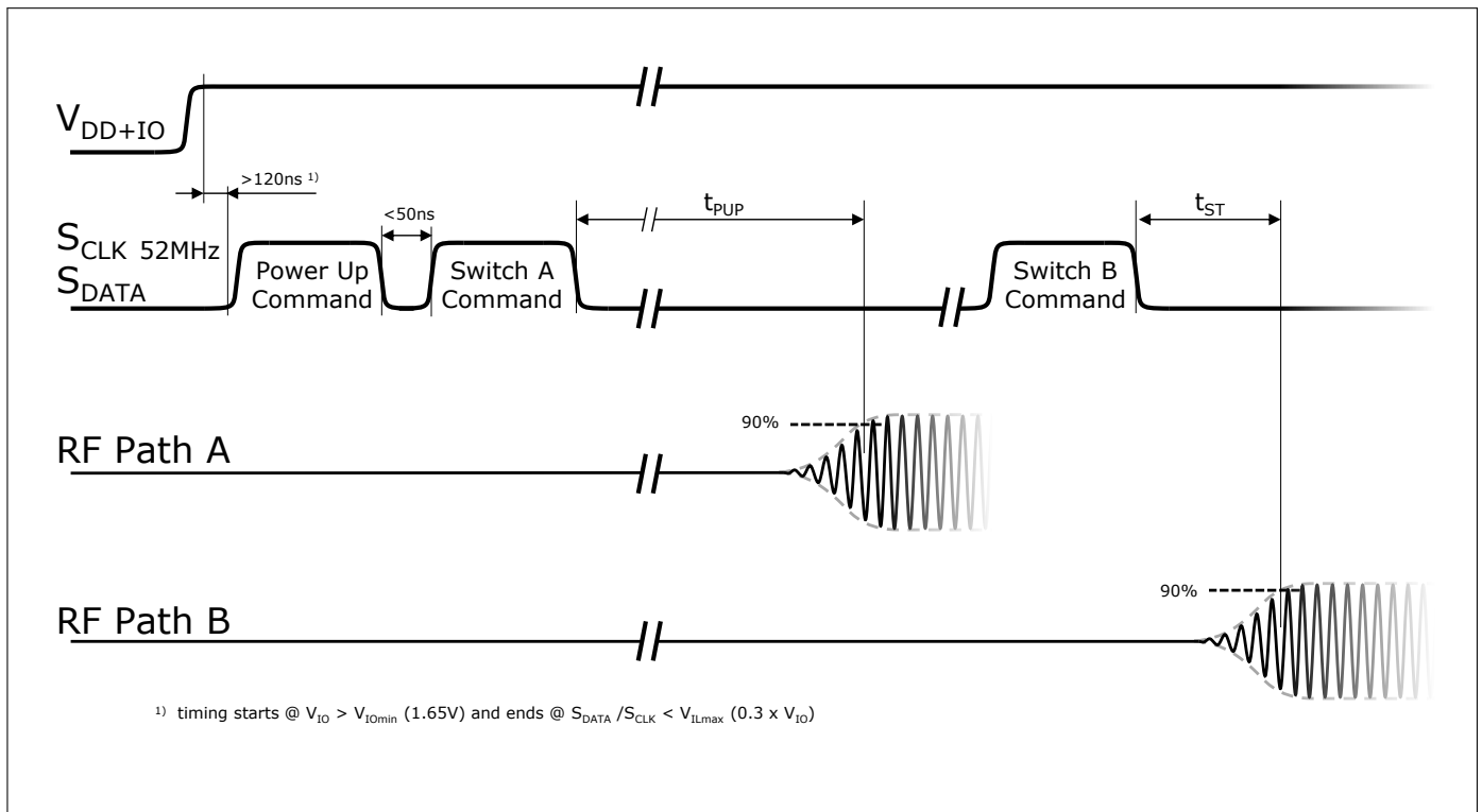
Figure 4: BGSA144ML10 Switching Time Behavior
