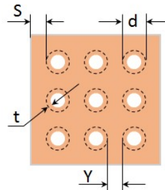
Figure 11 Thermal Via Pattern
