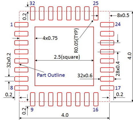
Figure 10 Stencil Openings (Dimensions are in mm)
