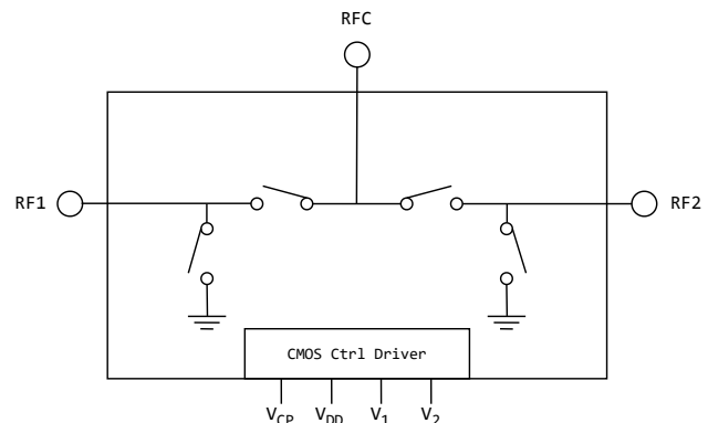
Figure 2: TS80220L functional diagram
