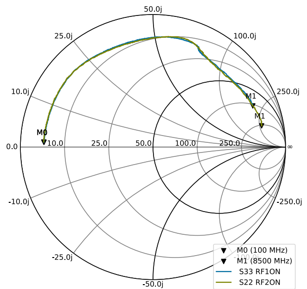
Non-active RF1 and RF2 termination impedance on Smith chart.
