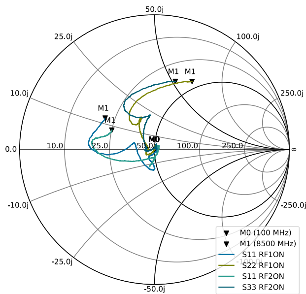
Active RF port impedance plotted to Smith chart
