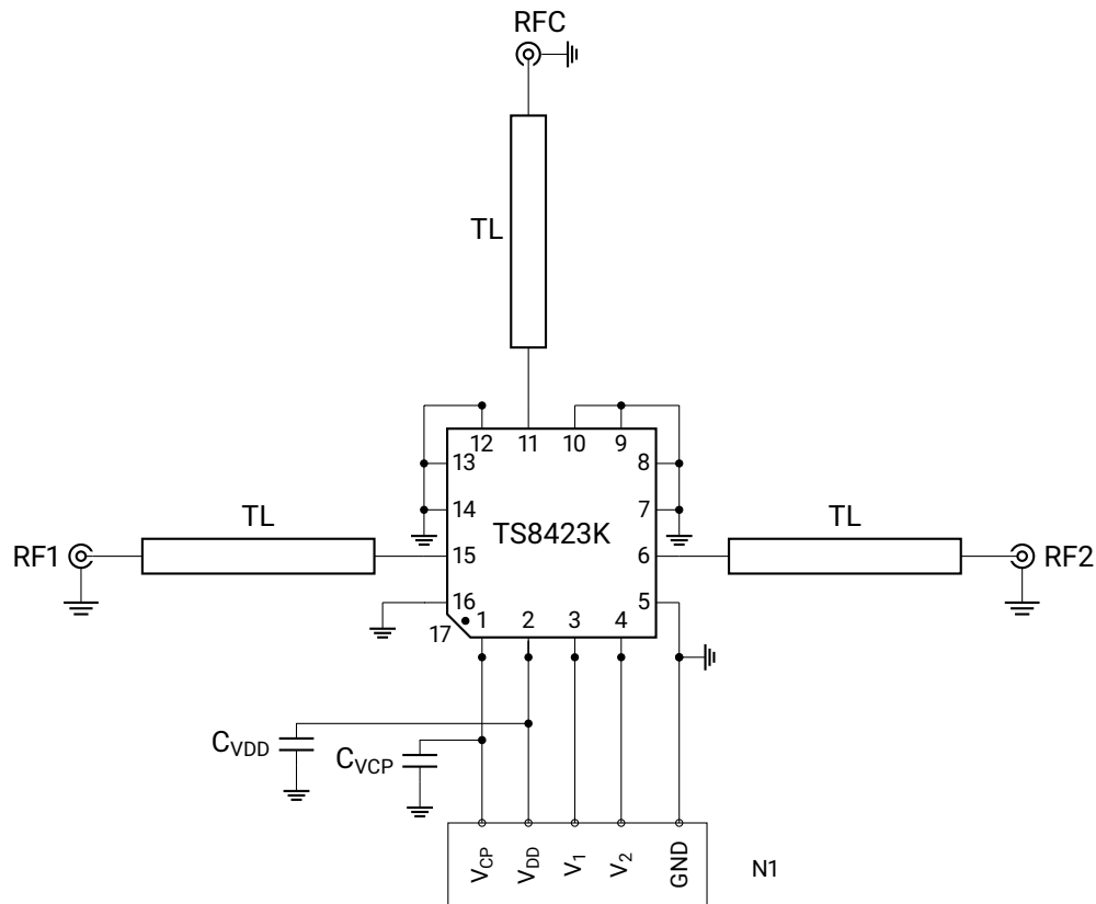
Schematics of TS8423K EVB
