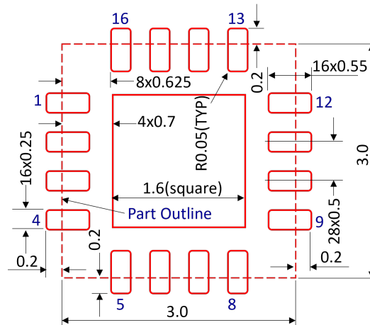
Figure 15: Stencil Openings, dimensions in [mm].
