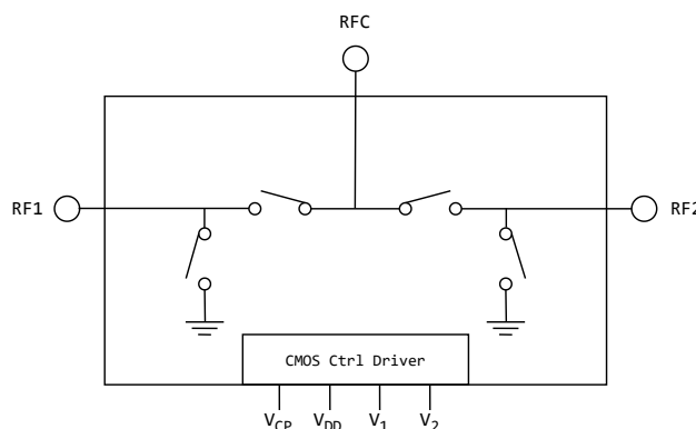
Figure 2: TS8423K functional diagram
