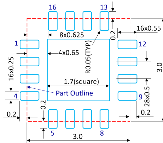
Figure 11: PCB land pattern, dimensions in [mm].
