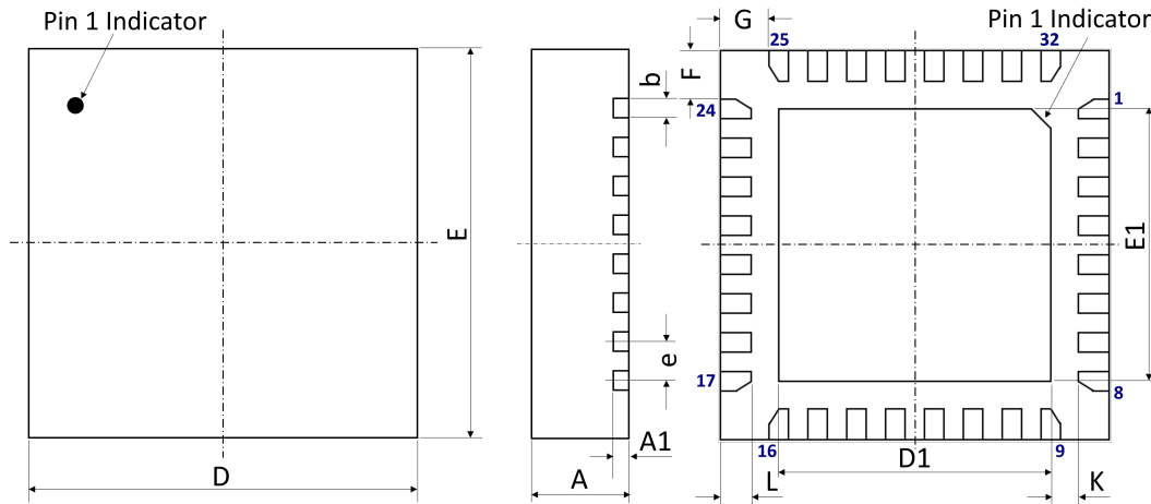
Figure 8: 32-pin QFN 5.0 x 5.0 x 0.85 mm 3 package drawing.
