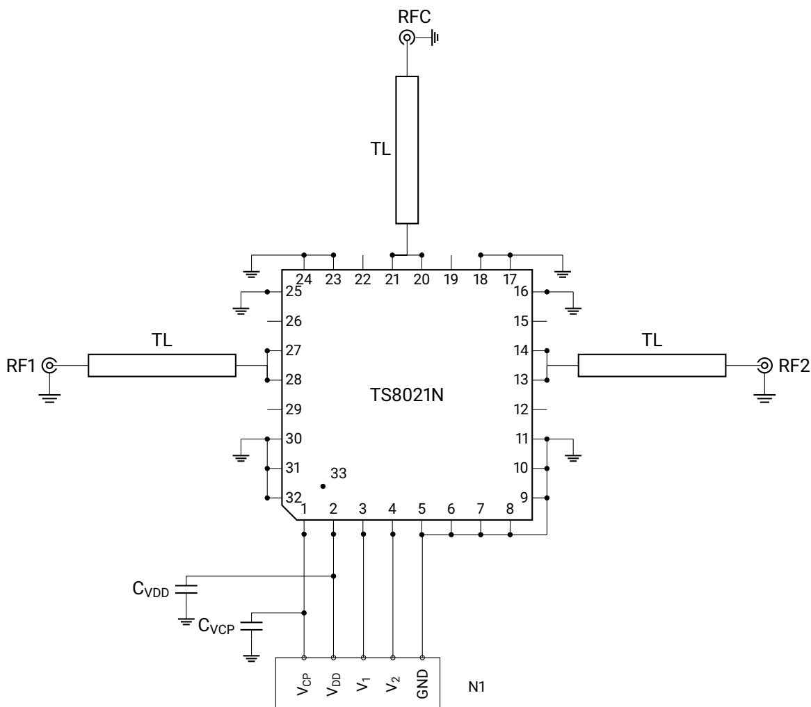
Schematics of TS8021N EVB with matching components
