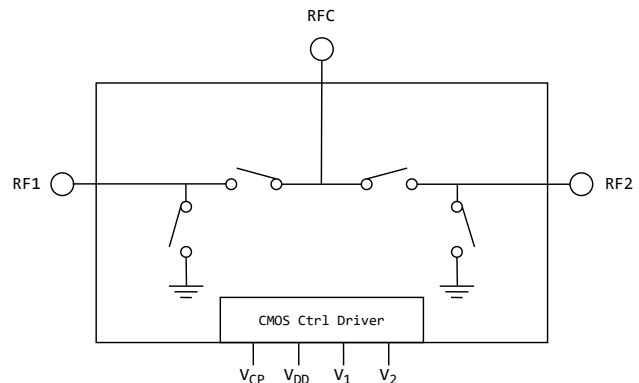
Figure 2: TS8021N functional diagram
