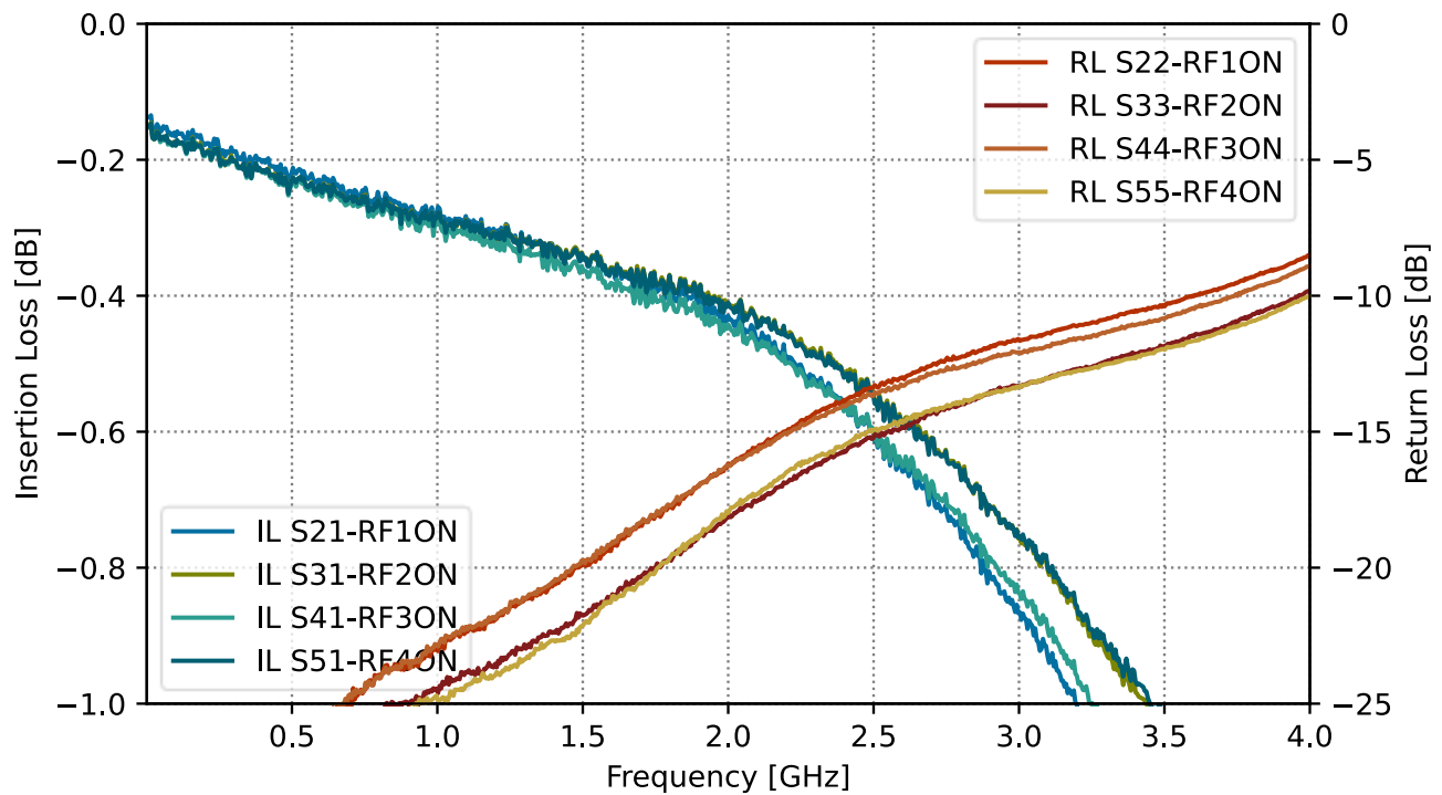
Figure 4 RF1 to RF4 Insertion Loss and Return Loss (no matching components on the EVB)
