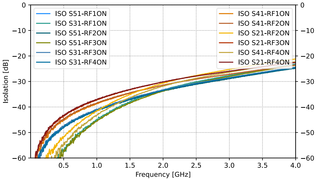
Figure 5 RFC to unused RF port isolations (no matching components on the EVB).
