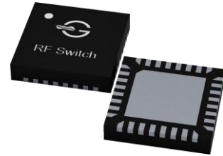
Figure 1 Device Image (32 Pin 4.0×4.0×0.75mm 3 QFN Package)
