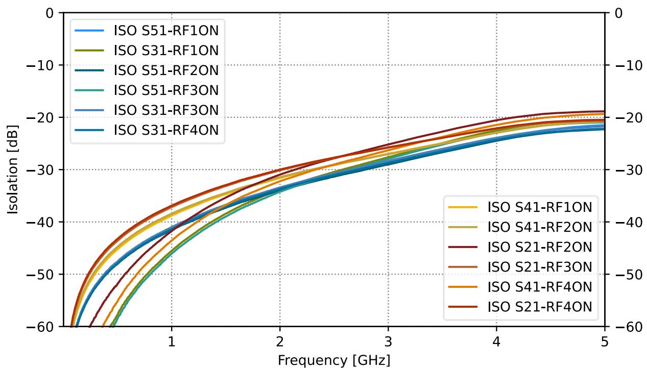
Figure 8 RFC to unused RF port isolations (matched upto 4300MHz)
