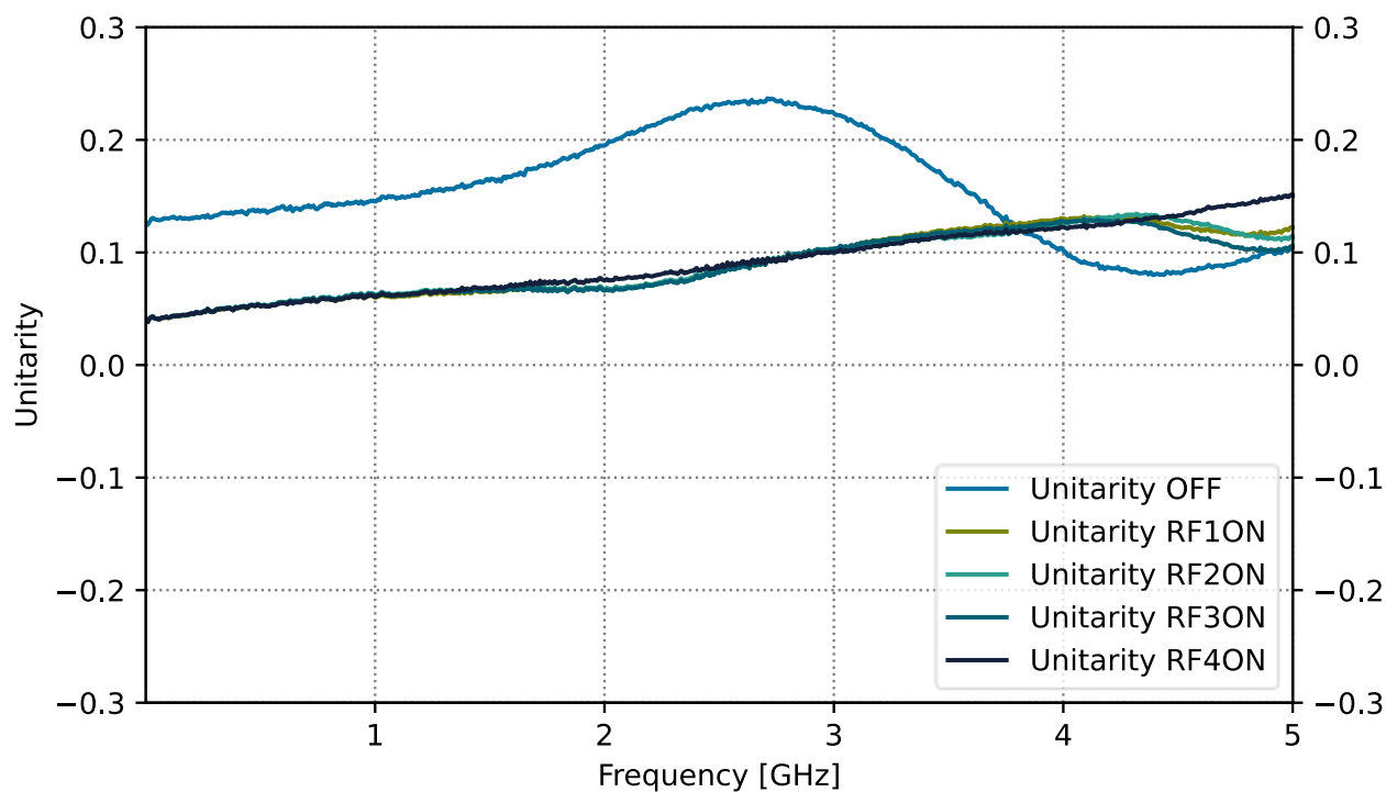
Figure 9 Unitarity (Power absorption of switch), matched upto 4300MHz
