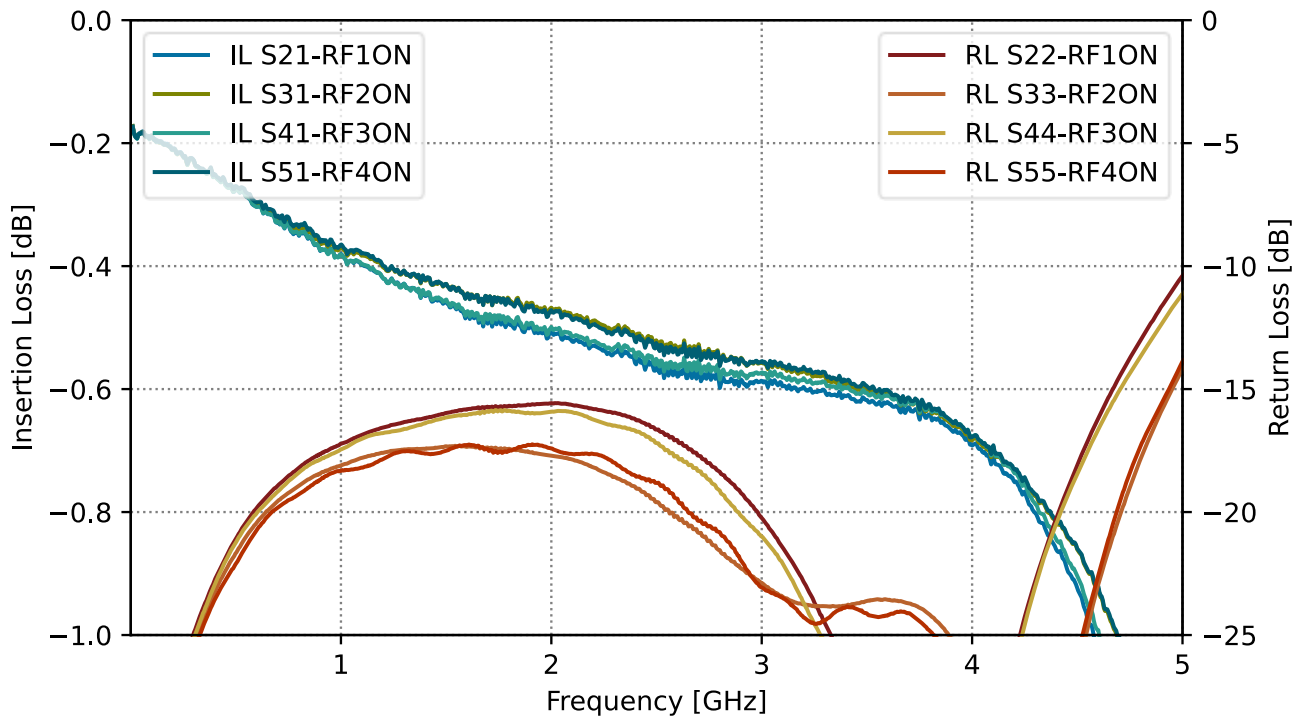
Figure 7 RF1 to RF4 Insertion Loss and Return Loss (matched upto 4300MHz)
