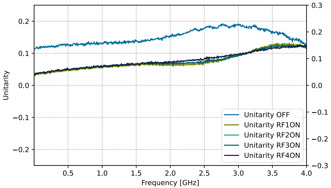
Figure 6 Unitarity (power absorption by RF Switch)
