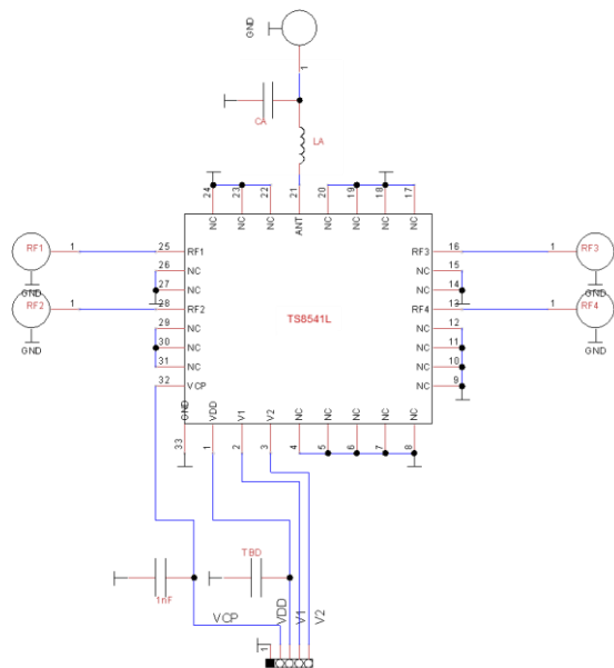
Figure 3 Evaluation Board Schematic and Picture (No Match)
