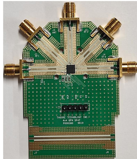
Figure 3 Evaluation Board Schematic and Picture (No Match)
