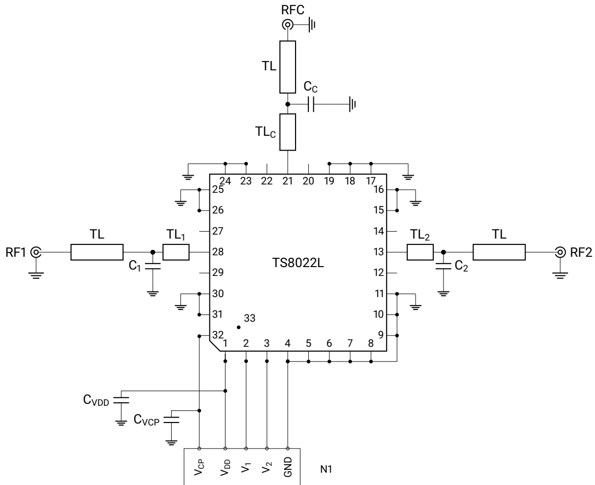
Schematics of TS8022L EVB with matching components
