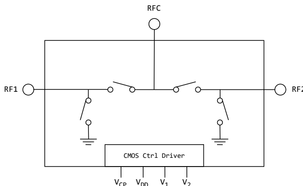
Figure 2: TS8022L functional diagram
