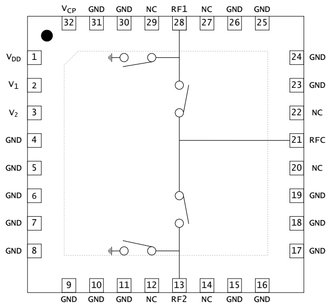
Figure 3: TS8022L pin assignment [top view]
