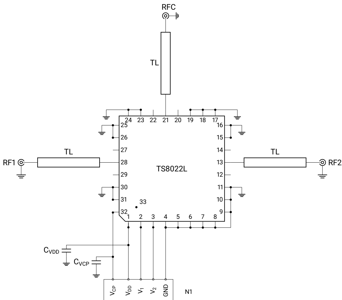
Schematics of TS8022L EVB
