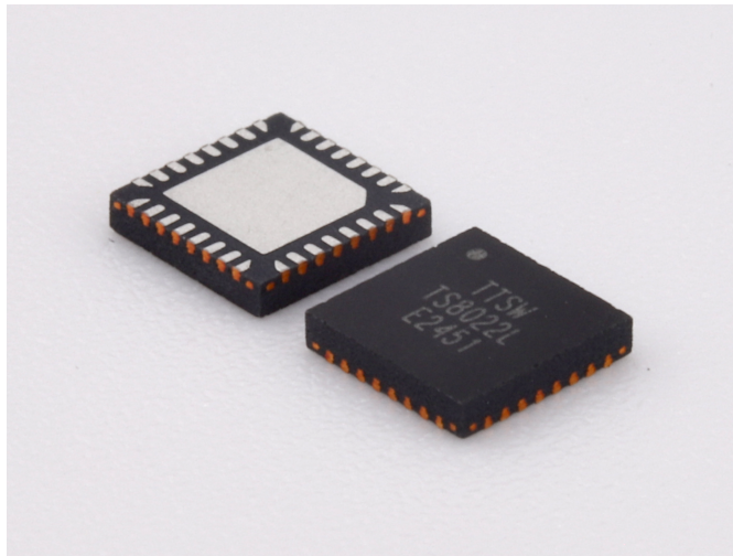
Figure 10: TS8022L photo, top and bottom side.
