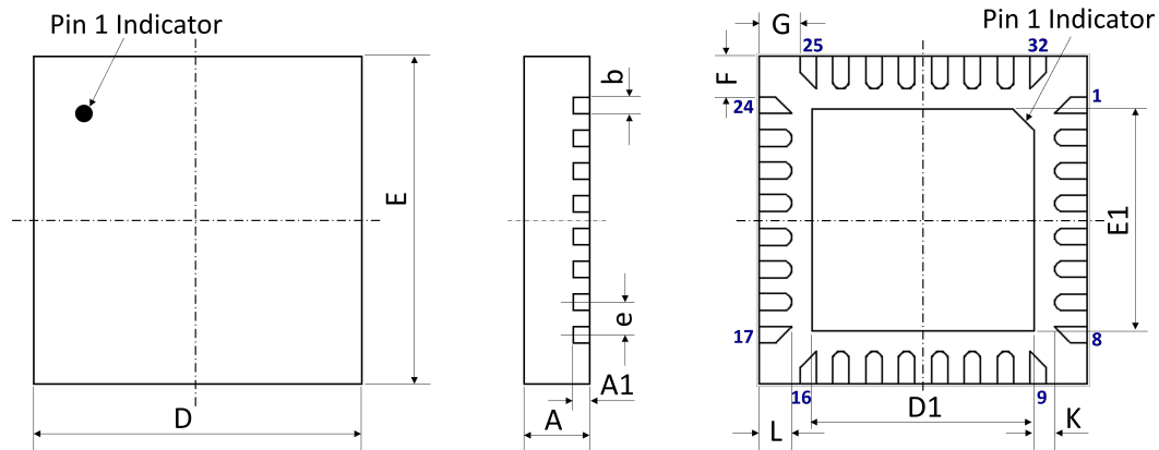
Figure 8: 32-pin QFN 4.0 x 4.0 x 0.85 mm 3 package drawing.
