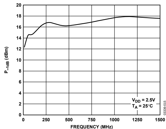
Figure 16. P_{-1\text{dB}} vs. Frequency
