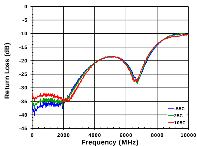
Figure 7. Return Loss vs. Frequency over Temp [RF2 Insertion Loss State]
