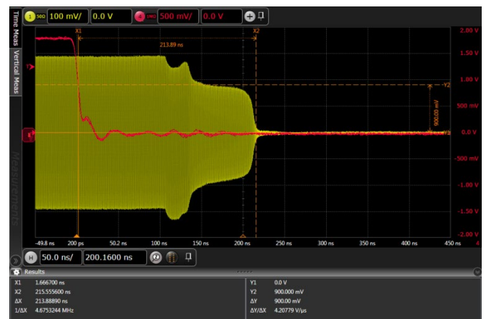
Figure 17. Switching Time Insertion Loss to Isolation
