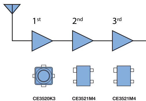
20GHz LNB
