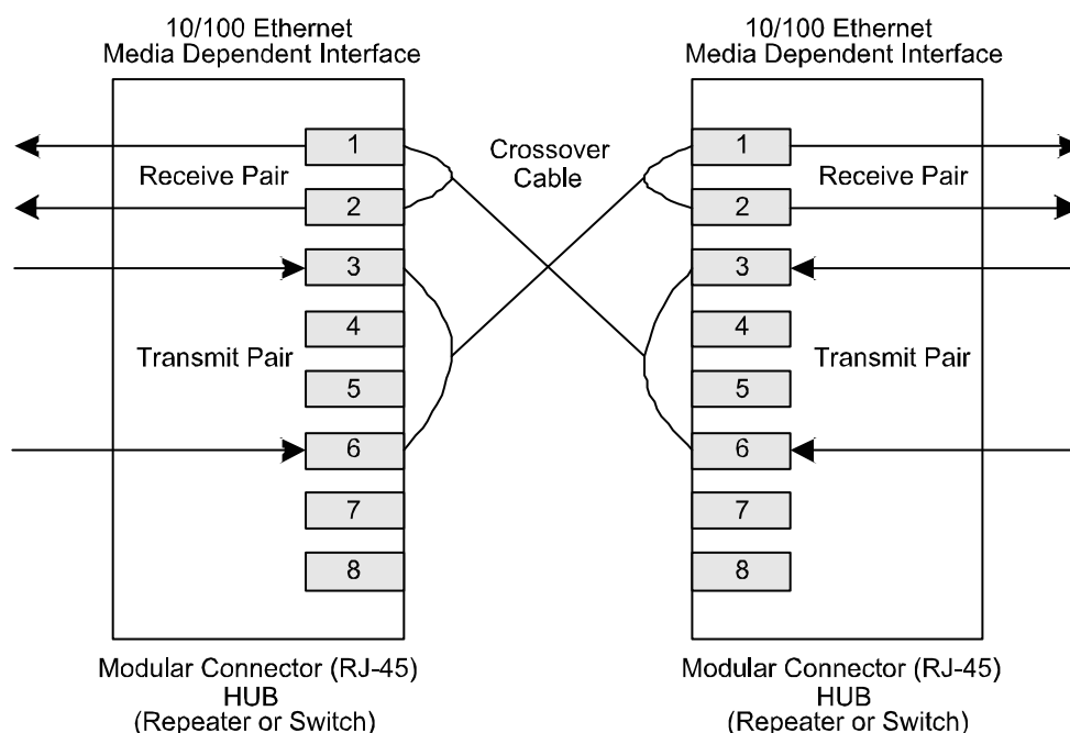
Figure 4. Typical Crossover Cable Connection
