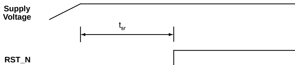
Figure 9. Reset Timing
