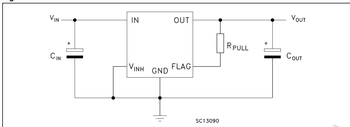
Figure 11. Test circuit
