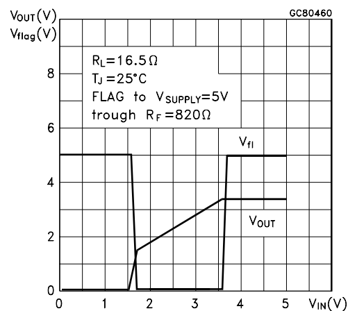
Figure 14. Output and flag voltage vs input
