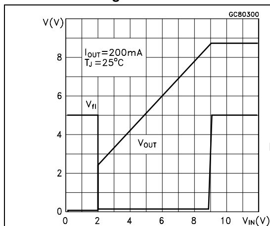
Figure 5. Output and flag voltage vs input voltage
