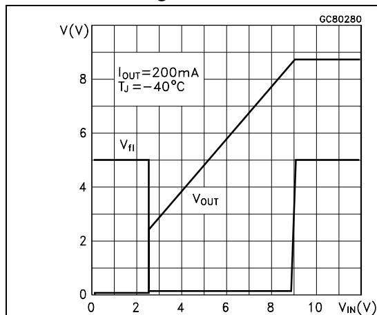
Figure 5. Output and flag voltage vs input voltage
