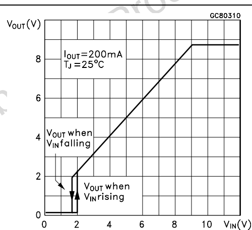
Figure 7. Output and flag voltage vs inp. volt. Figure 8. Output voltage vs input voltage
