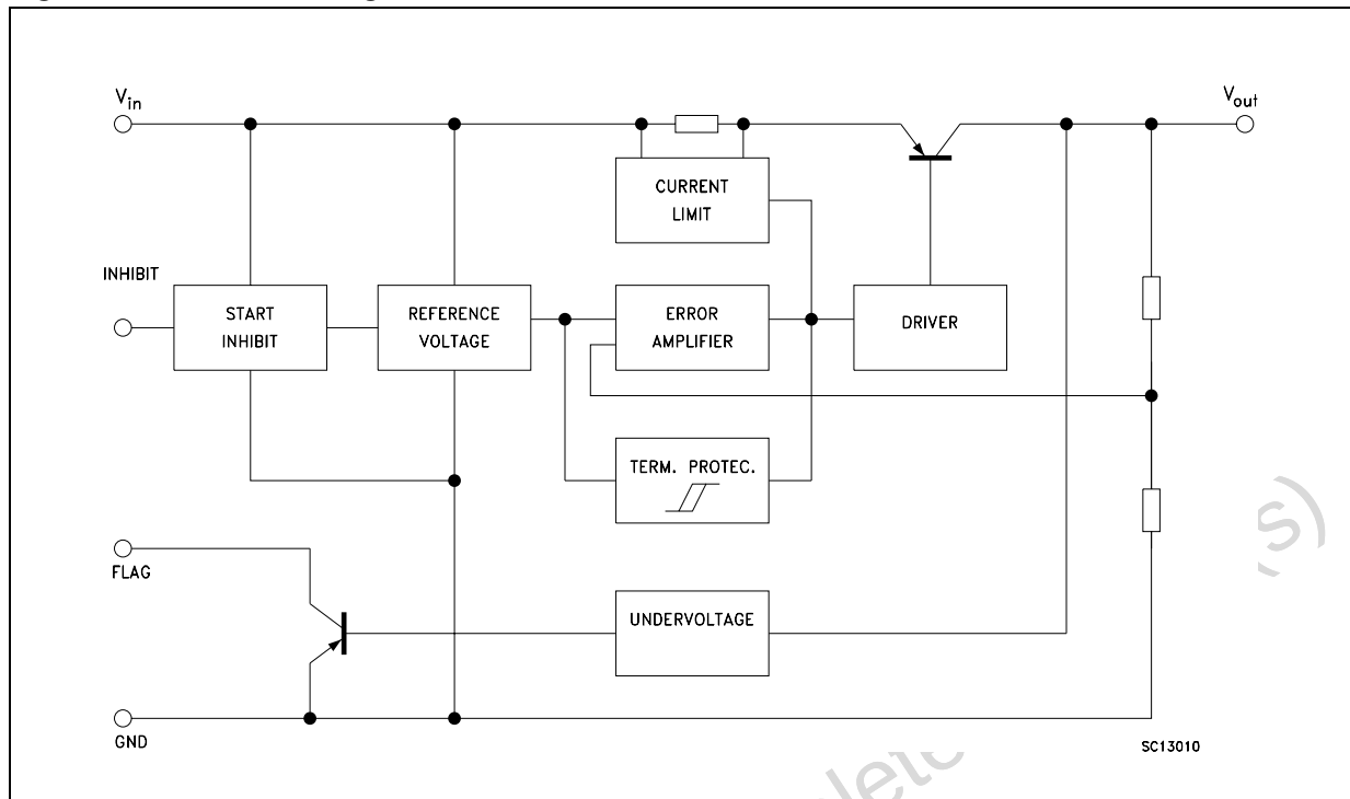
Figure 1. Schematic diagram
