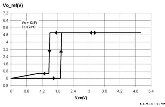
Figure 5. Output voltage vs V_{En}
