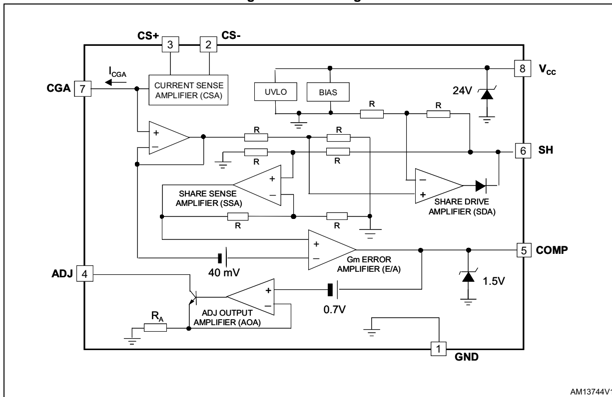
Figure 3. Block diagram
