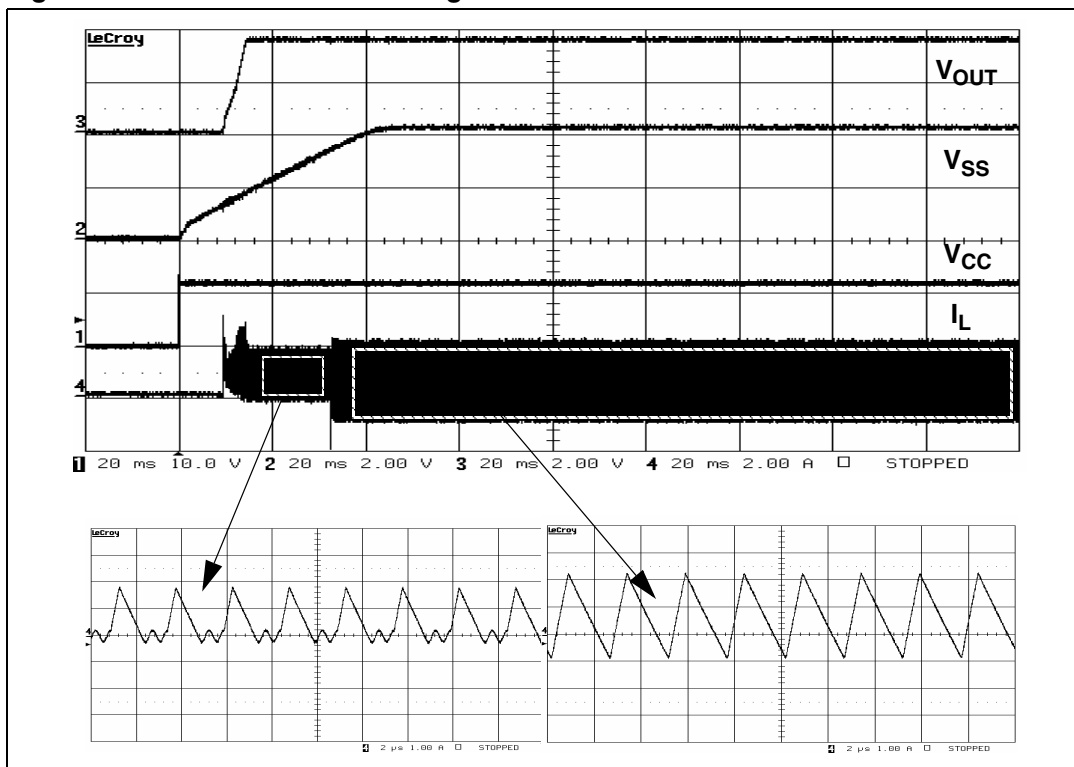
Figure 9. Inductor current during and after soft-start
