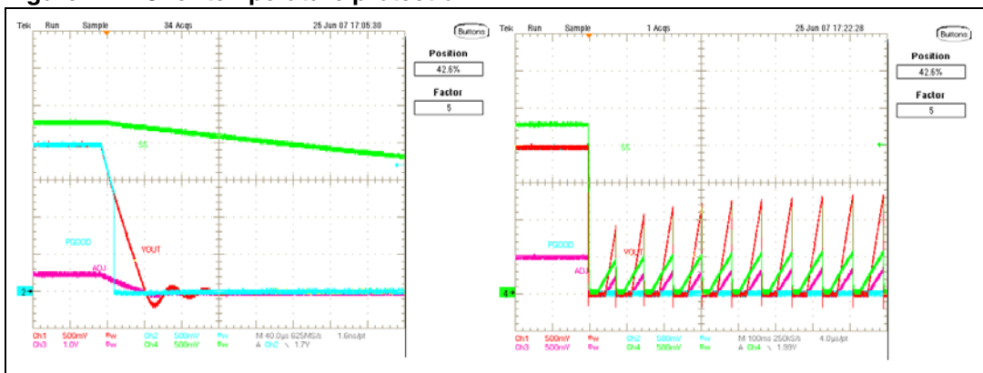
Figure 12. Over-temperature protection
