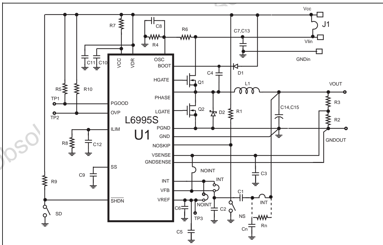
Figure 16. Schematic Diagram
