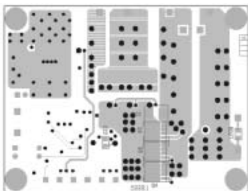
Figure 12. PCB Layout: Top side
