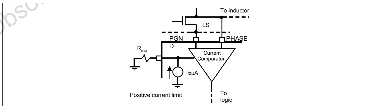
Figure 9. Current limit schematic
