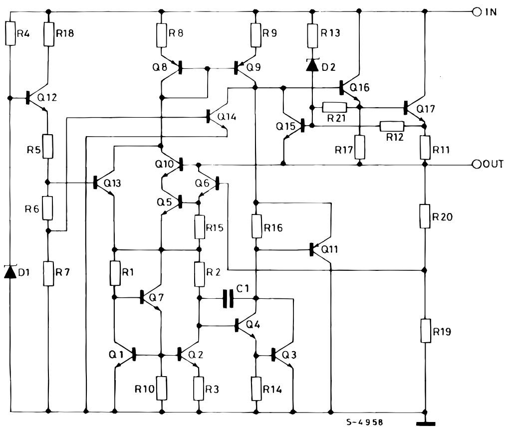
Figure 4. Schematic diagram
