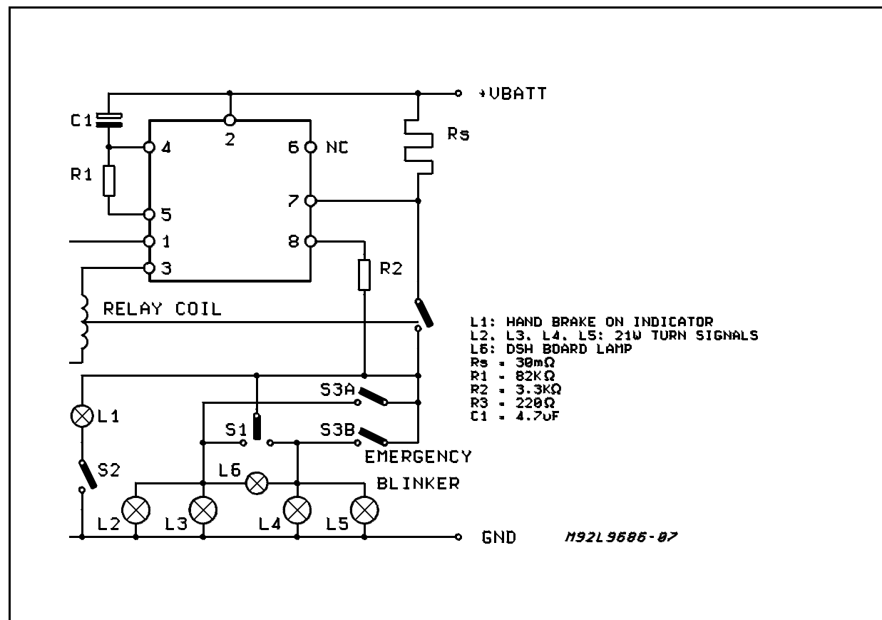
Figure 1: Application Circuit.
