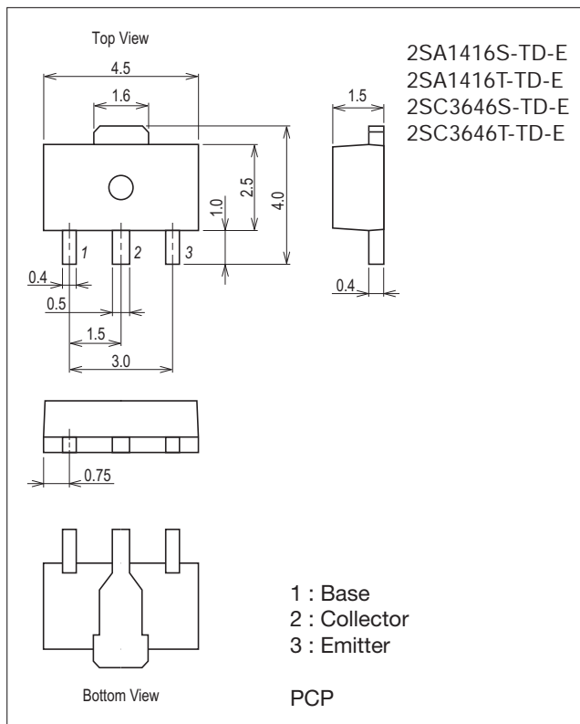
2SA1416
