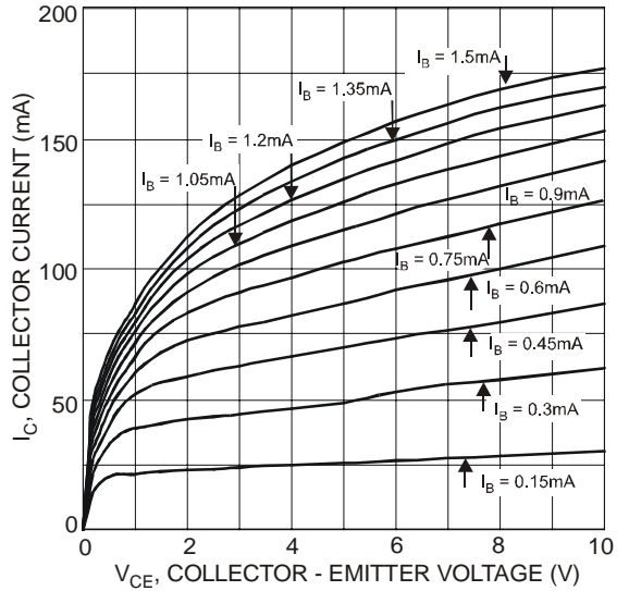
Fig. 10 Collector Current vs. Collector-Emitter Voltage
