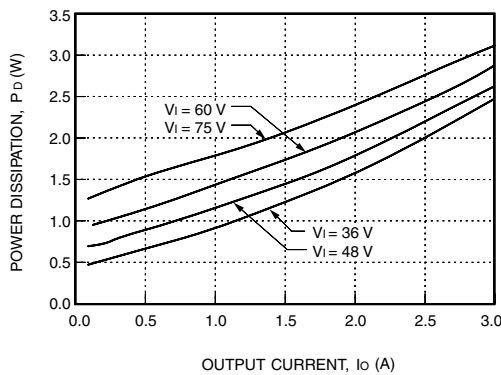
Figure 55. LW010D, LW015D Typical Power Dissipation vs. Output Current at T_c = 25^\circ C
