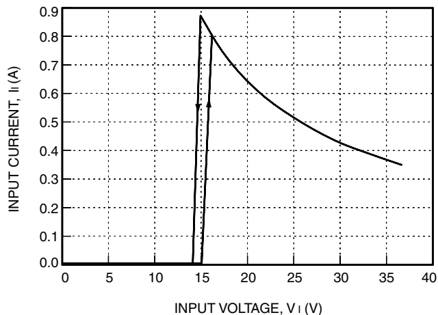
Figure 1. LC010 Input Current vs. Input Voltage at I_o = I_{o, max} and T_c = 25^\circ\text{C}
