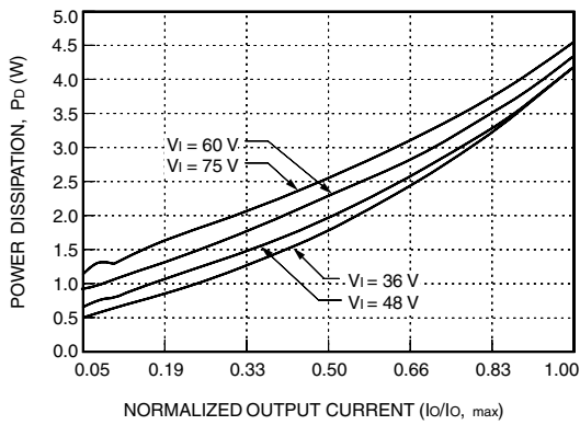
Figure 54. LW015B, C Typical Power Dissipation vs. Normalized Output Current at T_c = 25^\circ C
