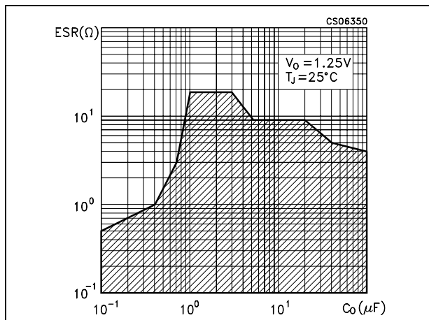
Figure 26. Stability
