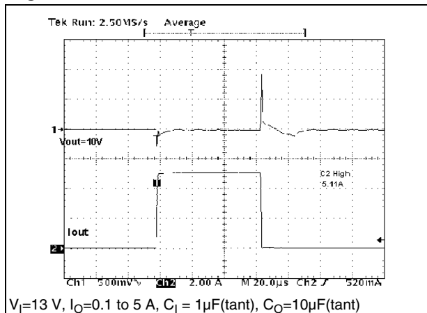
Figure 32. Load Transient
