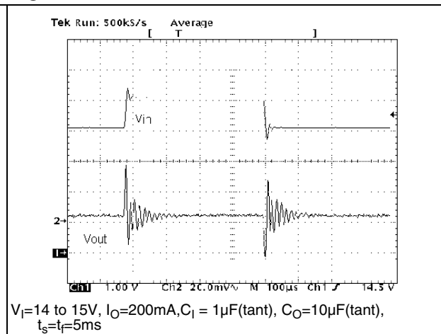
Figure 27. Line transient
