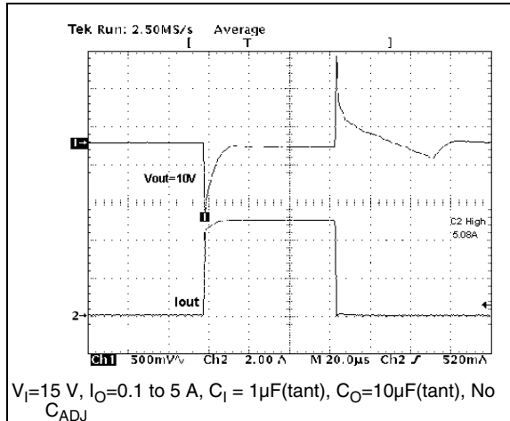
Figure 32. Load Transient
