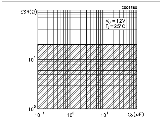
Figure 26. Stability
