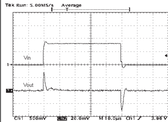
Figure 13. Line transient ( t_r = t_f = 500 \text{ ns} )
