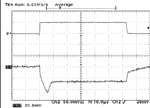
Figure 15. Load transient ( C_O = 10 \text{ µF} )
