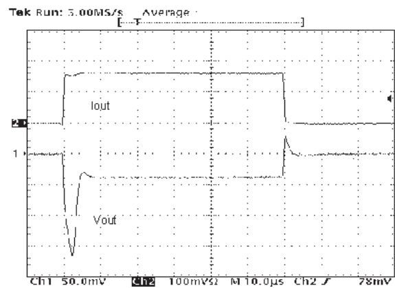
Figure 16. Load transient ( C_O = 4.7 \text{ µF} )
