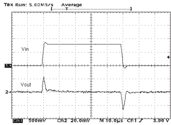
Figure 14. Line transient ( t_r = t_f = 1 \text{ µs} )
