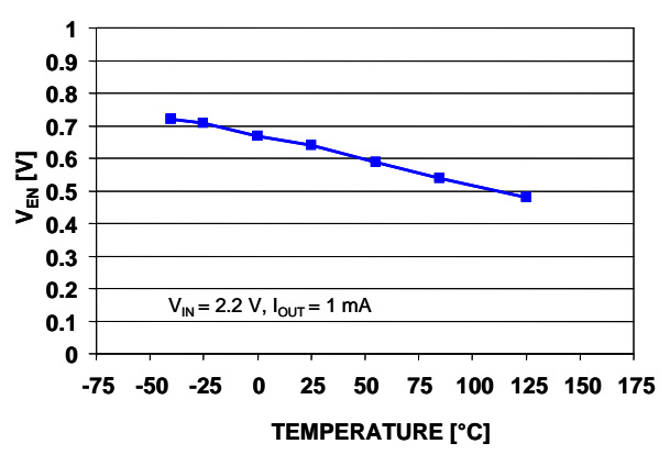
Figure 13. Enable threshold vs. temperature
