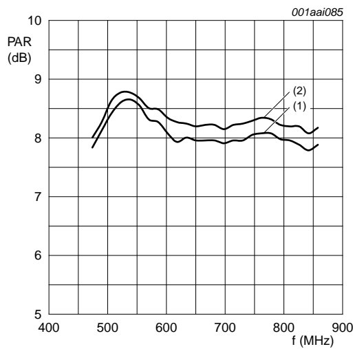
P_{L(AV)} = 77 W; I_{Dq} = 1.4 A; measured in a common source broadband test circuit as described in Section 8 . PAR of input signal = 9.5 dB at 0.01 % probability on CCDF. (1) V_{DS} = 40 V (2) V_{DS} = 42 V
