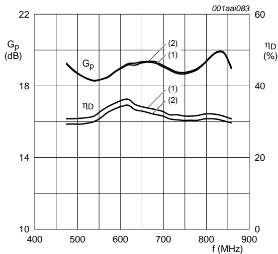
P_{L(AV)} = 77 W; I_{Dq} = 1.4 A; measured in a common source broadband test circuit as described in Section 8 . (1) V_{DS} = 40 V (2) V_{DS} = 42 V
