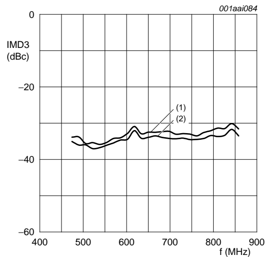
P_{L(AV)} = 77 W; I_{Dq} = 1.4 A; measured in a common source broadband test circuit as described in Section 8 . (1) V_{DS} = 40 V (2) V_{DS} = 42 V
