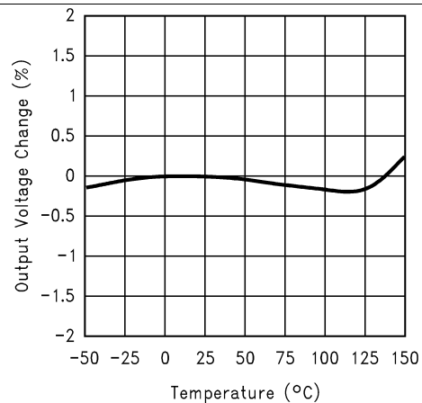
Figure 6. Temperature Stability
