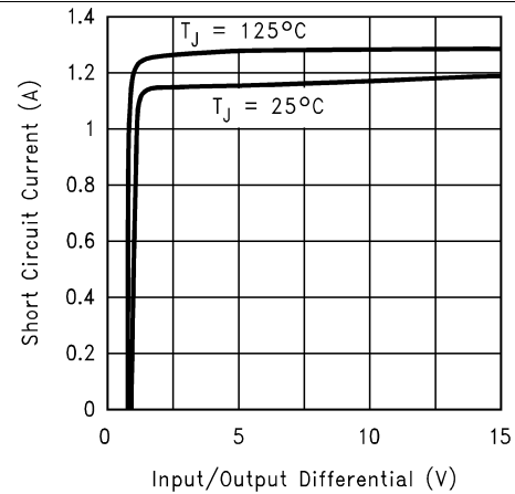
Figure 2. Short-Circuit Current
