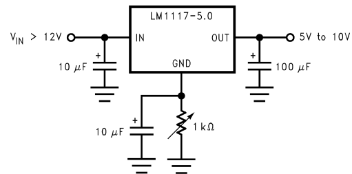
Figure 17. Adjusting Output of Fixed Regulators
