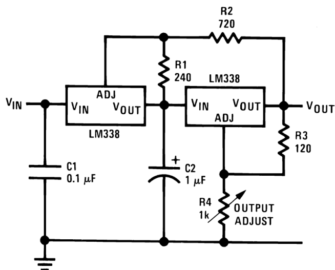
Figure 38. Tracking Preregulator
