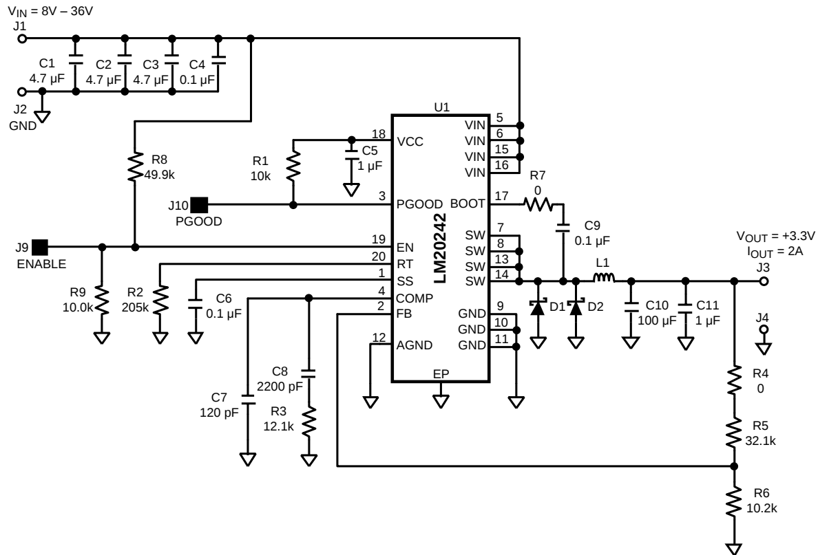
Figure 17. Typical Application Schematic
