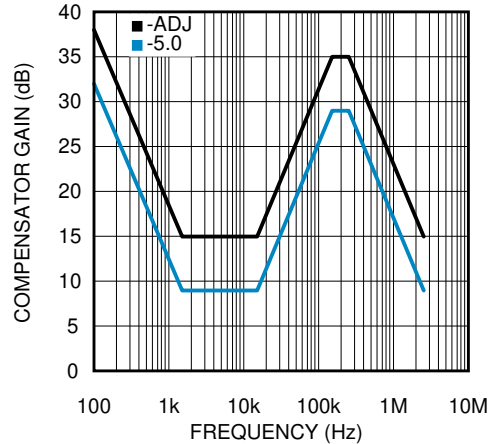
Figure 7-2. Compensator Gain
