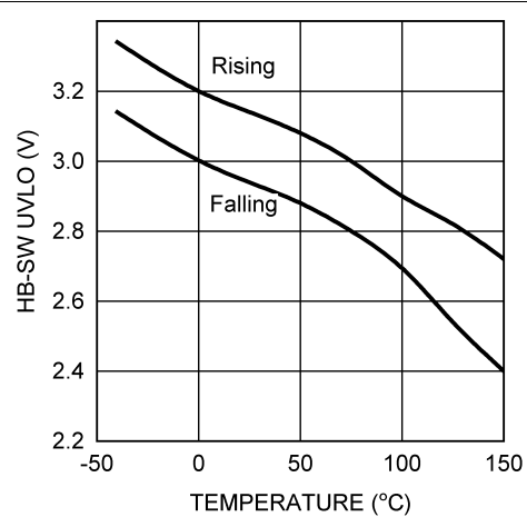
Figure 10. HB to SW UVLO vs Temperature
