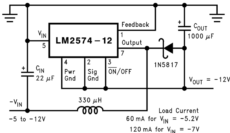
Figure 21. Negative Boost
