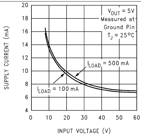
Figure 5. Supply Current
