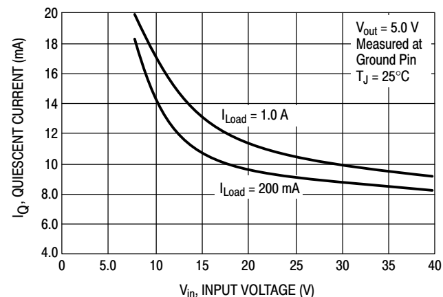
Figure 7. Quiescent Current
