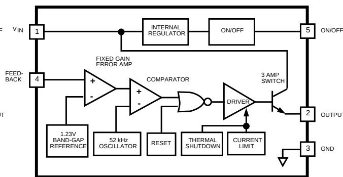
Adjustable Regulator
