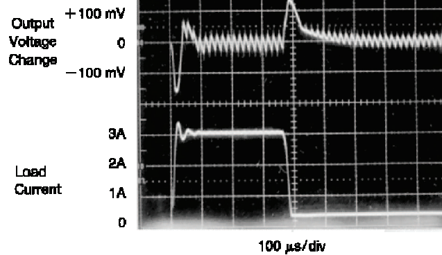
Figure 19. Load Transient Response
