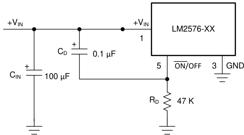
Figure 7-3. Delayed Start-Up
